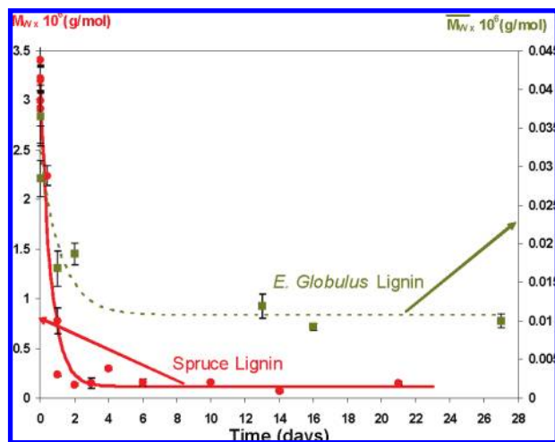
Figure 7. Incubation effect on the weight-average apparent molecular weight of the Norway spruce and Eucalyptus globulus lignin in THF solution maintained at room temperature.
