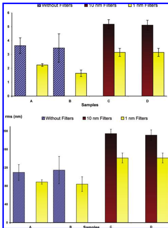
Figure 2. Effect of light scattering filters on the weight-average apparent molecular weight (top graph) and on the root-mean-square radius (bottom graph) of EMAL Norway spruce solutions in THF.
