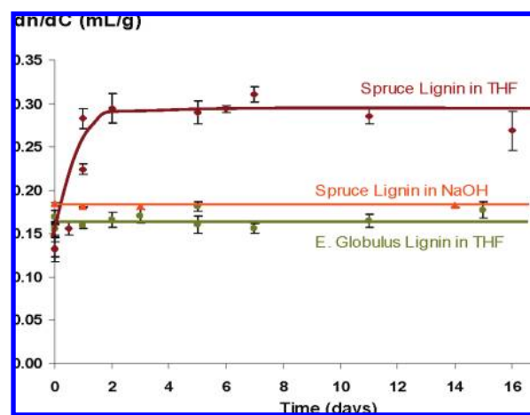
Figure 5. Incubation effect on the specific refractive index increment ( dn/dc ) of EMAL Norway spruce and Eucalyptus globulus in THF and EMAL Norway spruce lignin in 0.01 N NaOH.
