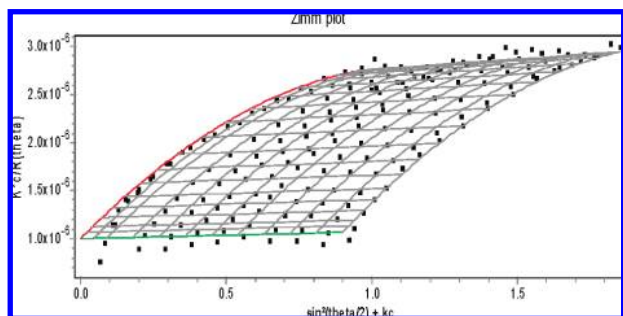
Figure 1. Typical Zimm plot by light scattering photometry from a Norway spruce lignin solution in THF.
