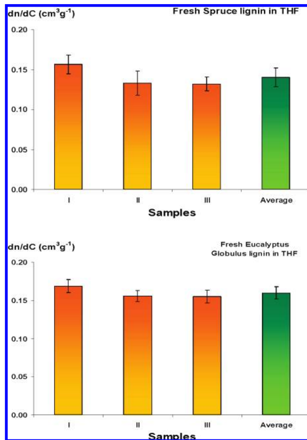
Figure 4. Reproducibility of the specific refractive index increment of fresh (just after dilution) EMAL Norway spruce solutions (top graph) and EMAL Eucalyptus globulus solutions (bottom graph), both in THF and at 25 °C.
